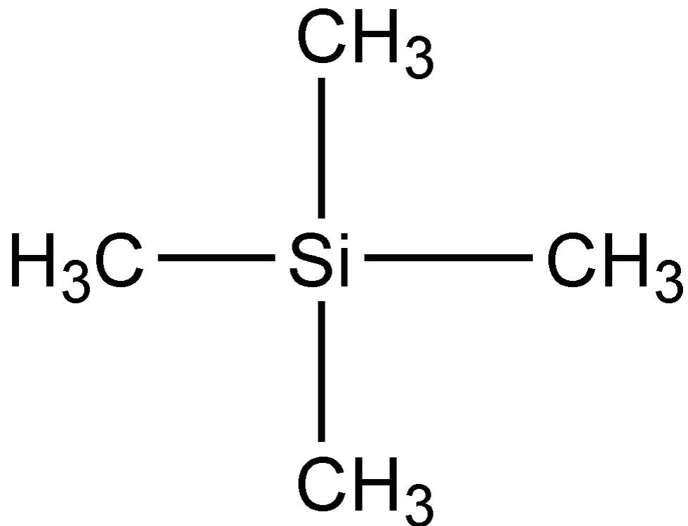
Abb. C-5 Tetramethylsilan, TMS
